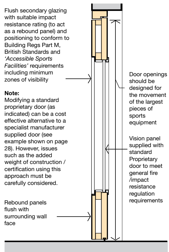
Store doors should be flush detailed, and unless they can only be opened by operators and otherwise kept locked, they should not open out into the sports hall. Doors may need to perform as rebound panels and therefore their construction needs to be robust and safe for users. Net bags should have no projecting fittings/features that could create a hazard and be high enough to not compromise the five-a-side rebound zone (1.21 m).
