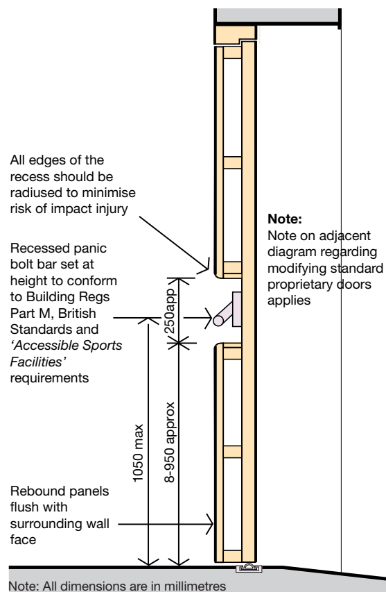
Sports hall walls should be detailed for safety and without hazardous projections. Flush surfaces should extend to 2.0 m minimum, preferably to 2.7 m above floor.
