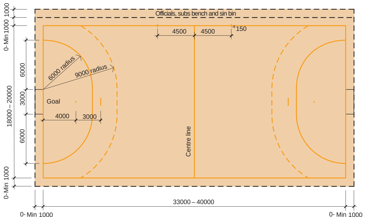
Dimensions of a handball court (mm)
