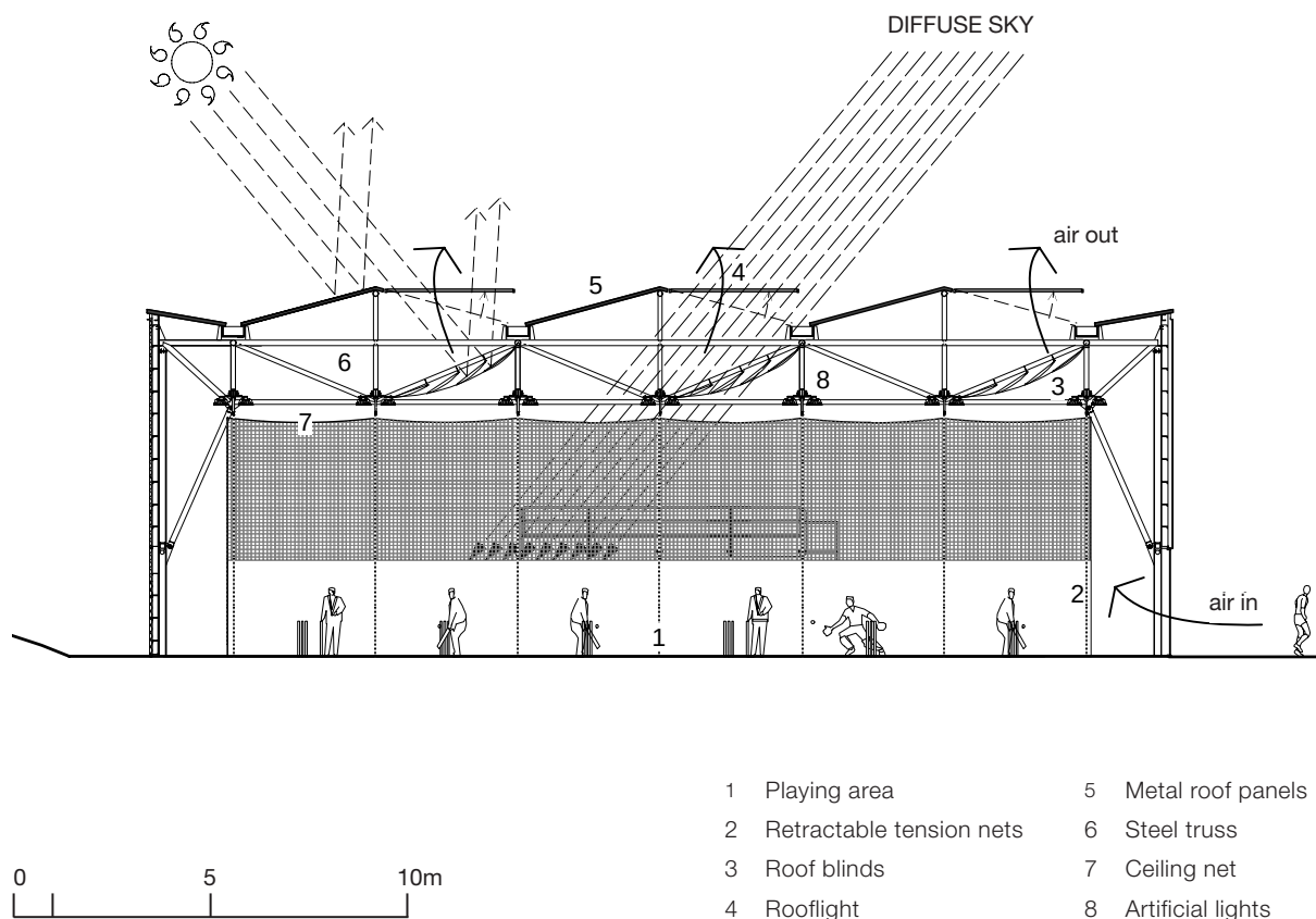
Example of daylighting successfully integrated into an indoor cricket school with north facing roof lights and screens to prevent entry of direct sunlight
