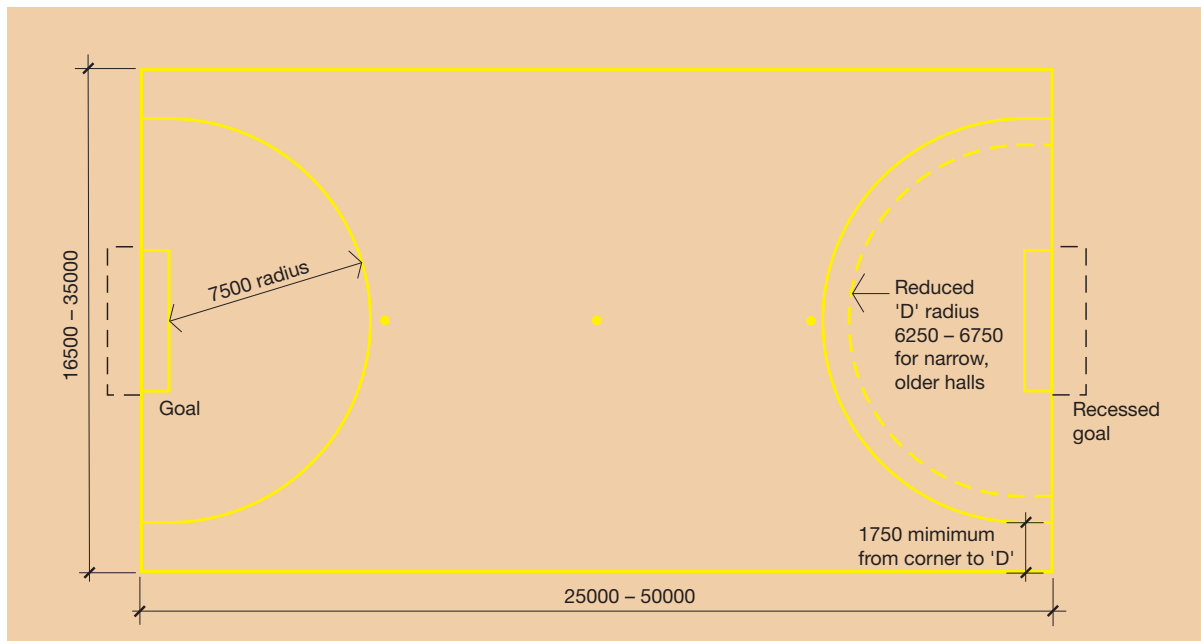
Dimensions of a five-a-side football pitch (mm)
